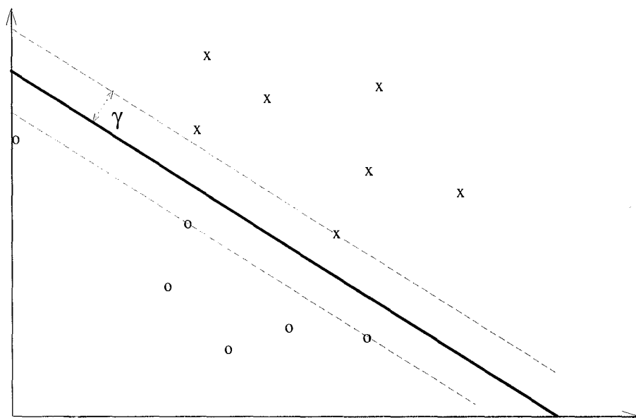
Figure 2.3: The margin of a training set
