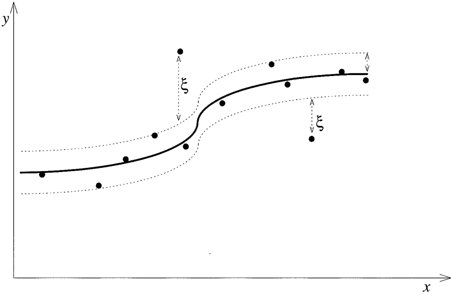
Figure 4.2: The slack variables for a non-linear regression function
