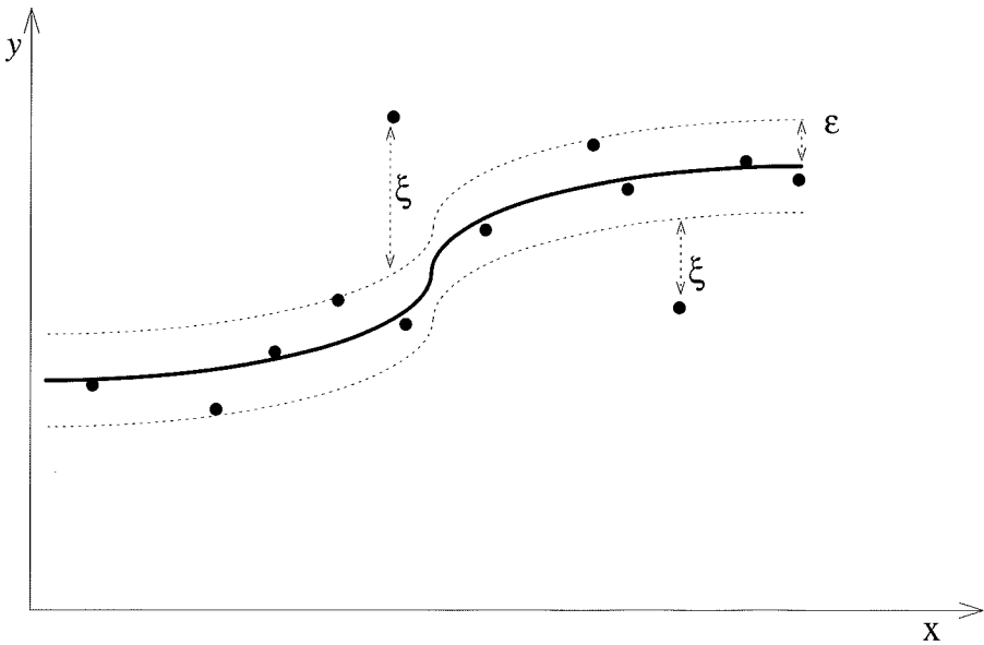
Figure 6.5: The insensitive band for a non-linear regression function
