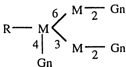
M 3 Gn 2 Gn b . Bisected bi-antennary complex
