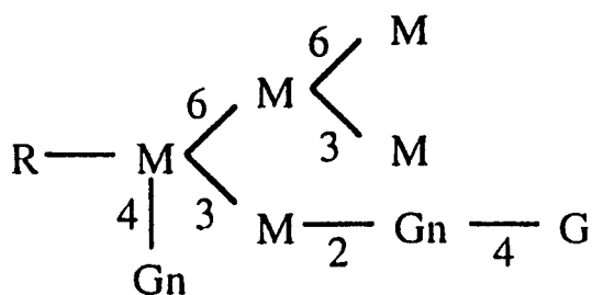
M 5 GnGn b G. Bisected hybrid
