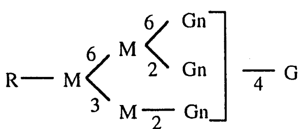
M 3 Gn 3 'G. Tri'-antennary complex
