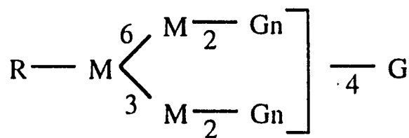
M 3 Gn 2 G. Bi-antennary complex
