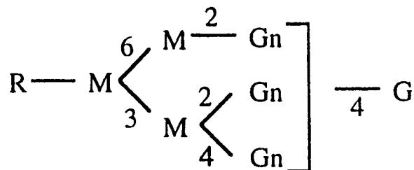
M 3 Gn 3 G. Tri-antennary complex
