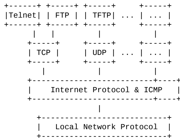
Protocol Relationships
