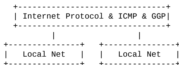
Gateway Protocols
