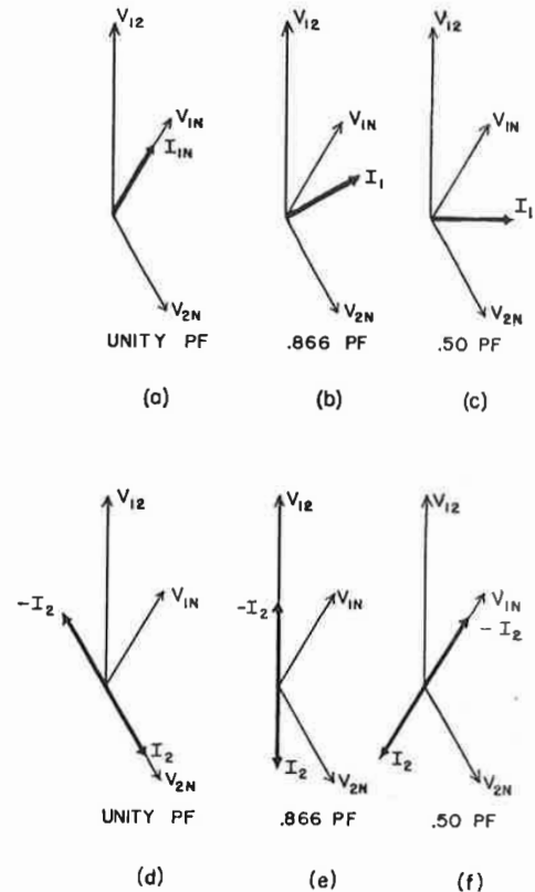
Fig. 17—Vector diagrams for various load power factors for metering line-to-neutral loads on two-phase, three-wire network circuit with a single-stator, three-wire meter.
