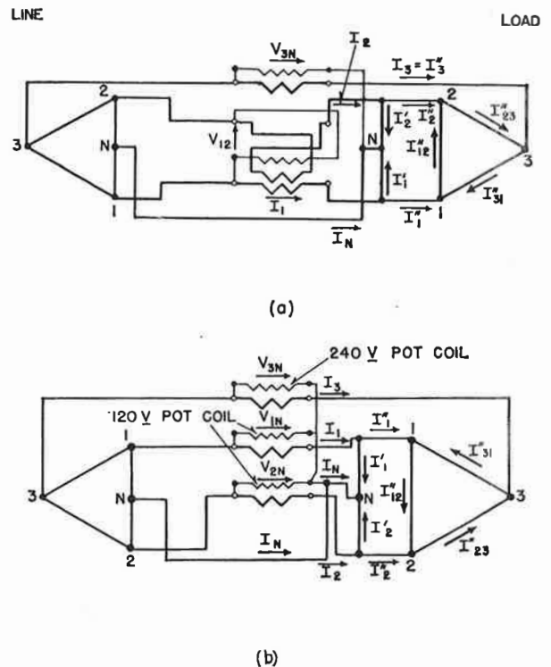
Fig. 22—Diagram of connections for metering a three-phase, four-wire delta circuit with (a) Two-stator meter, (b) Three-stator meter.
