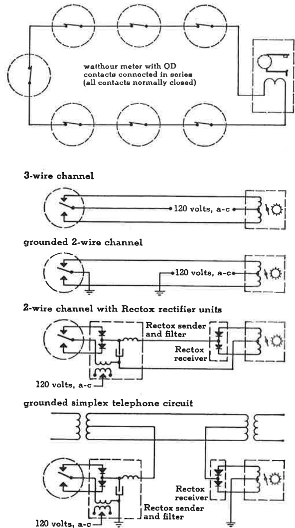
Fig. 44—Basic impulse totalization data transmission circuits.
