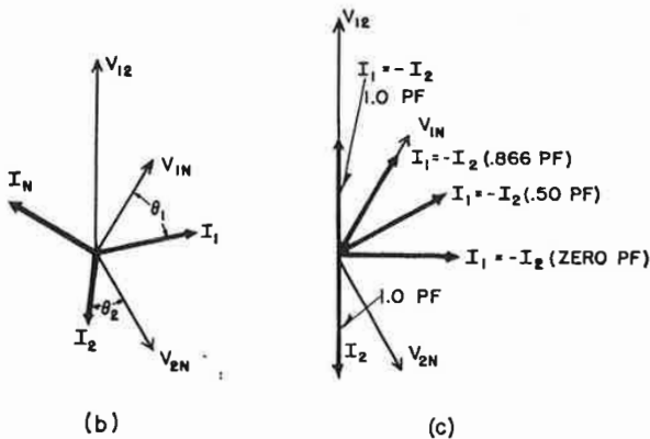
Fig. 15—Metering two-phase, three-wire network circuit, (a) Diagram of connections, (b) Vector diagram, balanced system voltages, unbalanced load, (c) Vector diagram for metering line-to-line loads, balanced system voltages.
