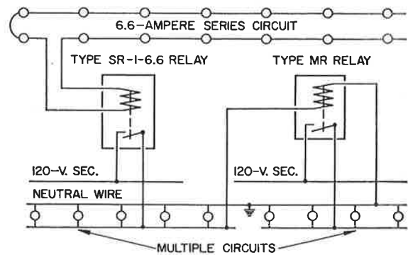
Fig. 23—A series-multiple street-lighting system using a type SR-1-6.6 series-multiple relay to switch the multiple lamps, and a type MR multiple relay to switch additional multiple lamp groups.
