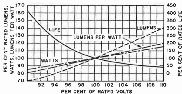
Fig. 2—Characteristic curves for incandescent lamps operated on a multiple circuit.
