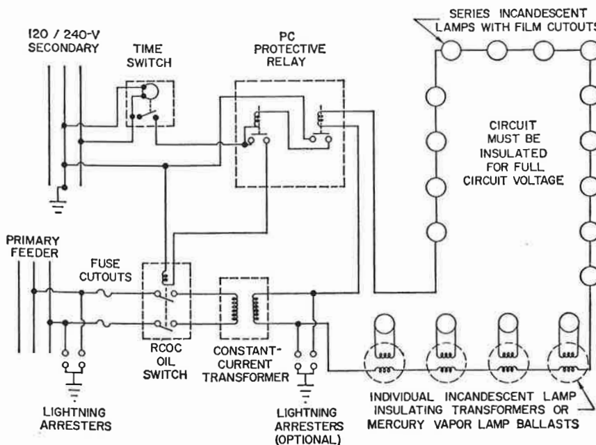
Fig. 13—Schematic diagram of a series street-lighting circuit.
