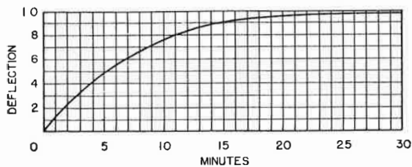
Fig. 36—Response characteristic of thermal demand meter.
