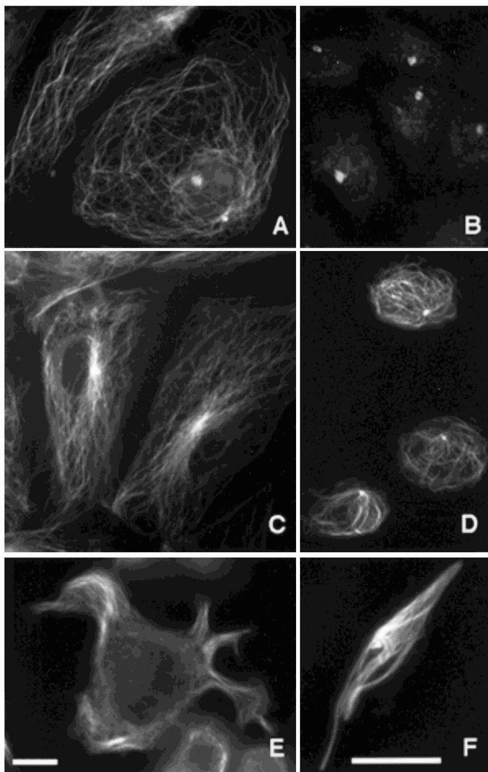
Fig. 8. Specific visualization of cellular microtubules with FLUTAX. A: PtK2 cytoskeletons (Fig. 5) were not fixed, but were incubated with 1 \mu M FLUTAX for 1 hr. Similar images were obtained at approximately 1 min after the addition of FLUTAX (not shown). B: Same as A, but with the addition of 50 \mu M docetaxel; Incubation with 2-Ac-FLUTAX gave a similar image (not shown). C: PtK2 cells incubated with 0.5 \mu M FLUTAX for 20 hr and directly mounted. D: U937 cells incubated with 37 nM FLUTAX for 16 hr. E: Neuro2A cells incubated with 1 \mu M FLUTAX for 2 hr. F: Trypanosoma cruzi epimastigotes incubated with 1 \mu M FLUTAX for 3 hr. Note that images (C–F)
