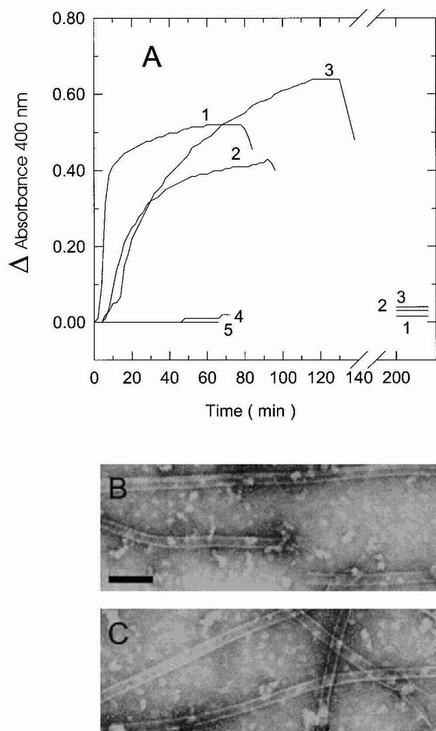
Fig. 2. Microtubule assembly induced by fluorescent taxoids. A: Turbidimetric records of 25 \mu M purified GDP-tubulin in PEGM buffer, pH 6.6 at 37°C, assembled with 30 \mu M taxol (1), FLUTAX (2), ROTAX (3), N-(4-fluoresceincarbonyl)-L-alanine methyl ester (4) or 2-Ac-FLUTAX (5). B: Electron micrograph of microtubules assembled with FLUTAX, negatively stained with uranyl acetate. C: Microtubules assembled with ROTAX. Bar = 100 nm.
