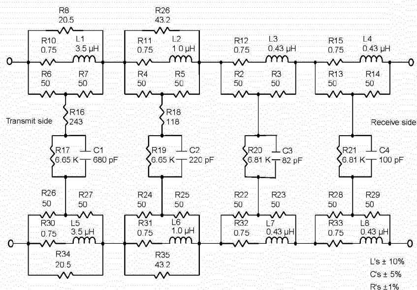
Figure 23-23—Worst-case UTP model
