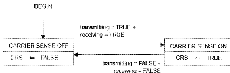
Figure 24-12—Carrier Sense state diagram
