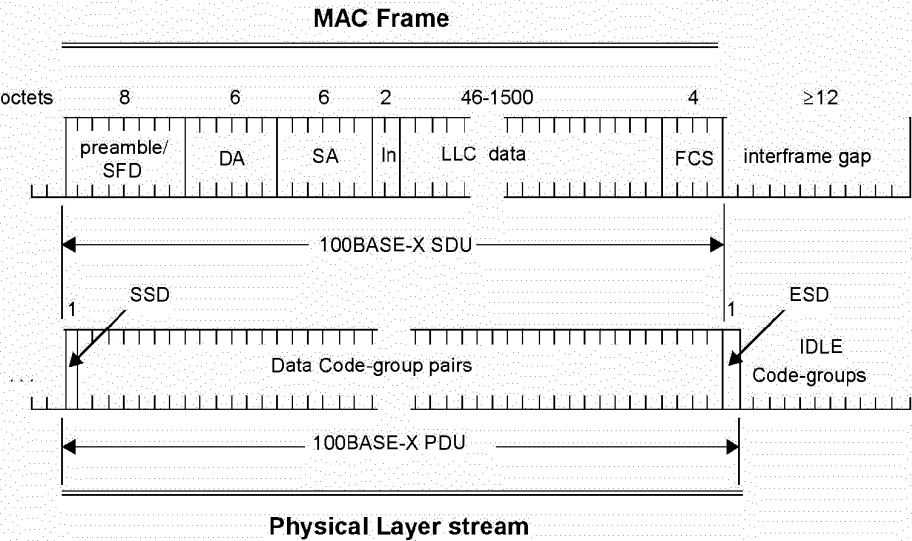
Figure 24-5—PCS encapsulation
