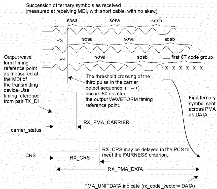
Figure 23-33—PMA RECEIVE timing start of packet
