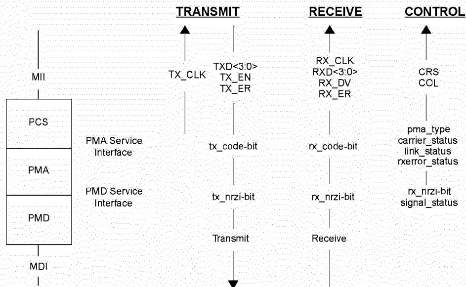
Figure 24-3—Interface mapping
