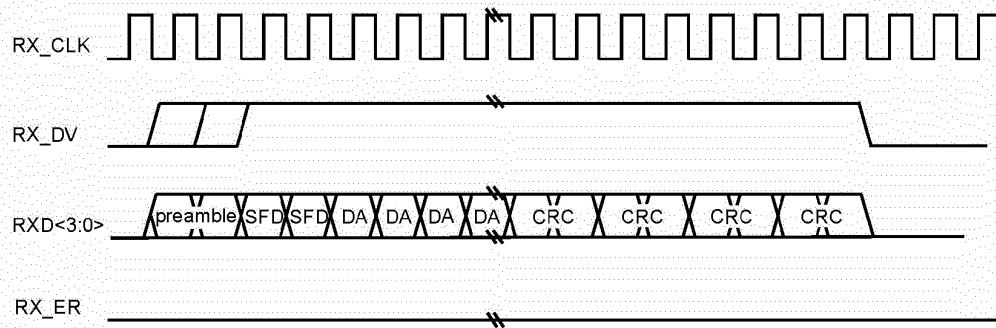
Figure 22-6—Reception with no errors
