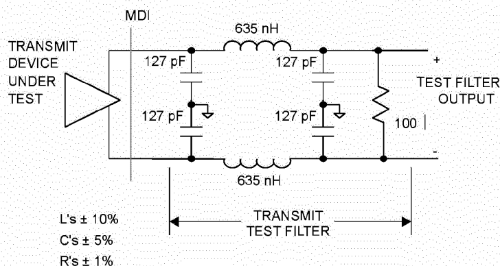
Figure 23-16—Acceptable implementation of transmit test filter
