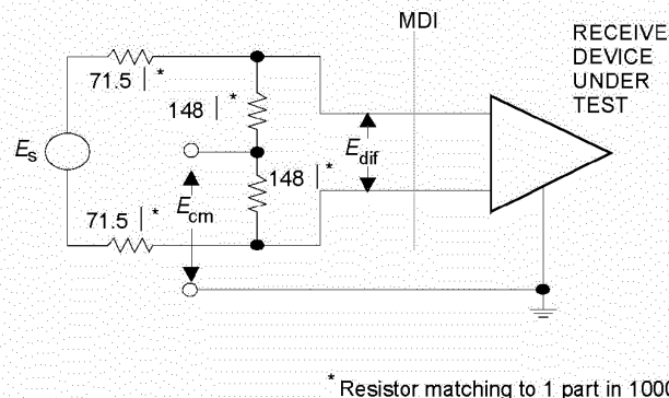
Figure 23-24—Receiver common-mode rejection test circuit
