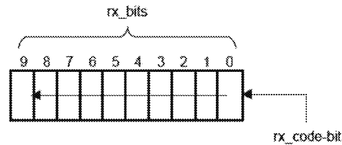
Figure 24-9—Receive Bits reference diagram
