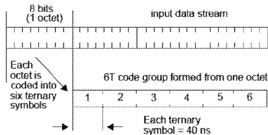
Figure 23-4—8B6T coding
