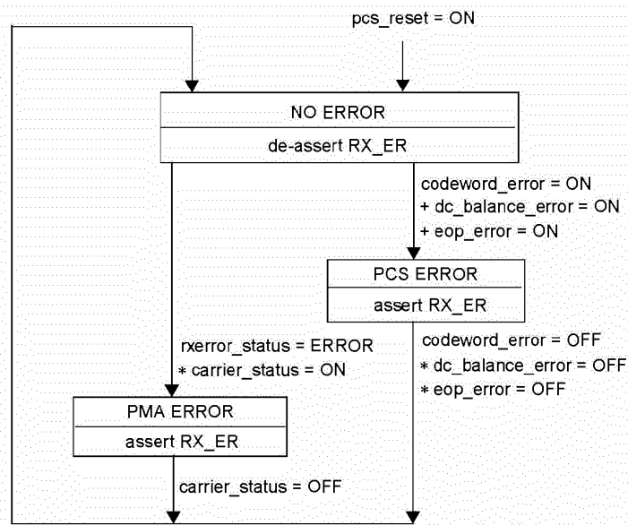
Figure 23-10—PCS Error Sense state diagram
