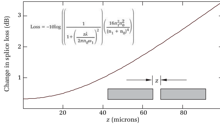
Figure 2.17. Coupling loss in single-mode fiber as a function of longitudinal misalignment. The mode-field diameter for both fibers is 4.5 \mu\text{m} , and the core index is 1.468. The index of air is 1. Nonzero loss at 0- \mu\text{m} misalignment is caused by surface reflections (interference effects are not included).
