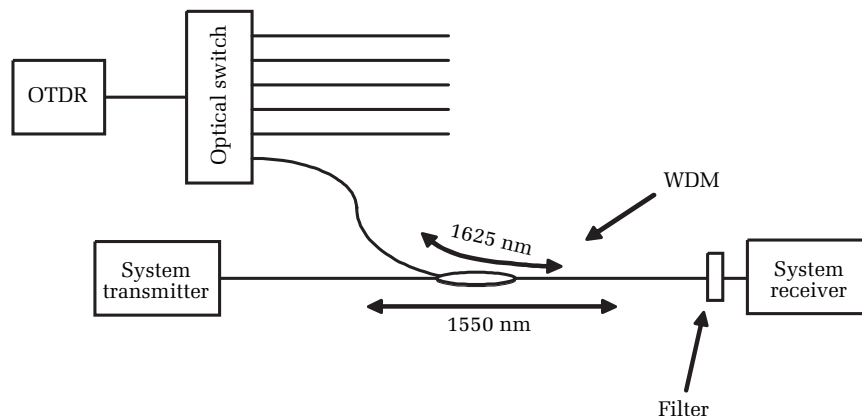
Figure 11.17. Remote OTDR testing on live optical fibers, using a WDM and optical filter to prevent the OTDR and system from interfering with each other.
