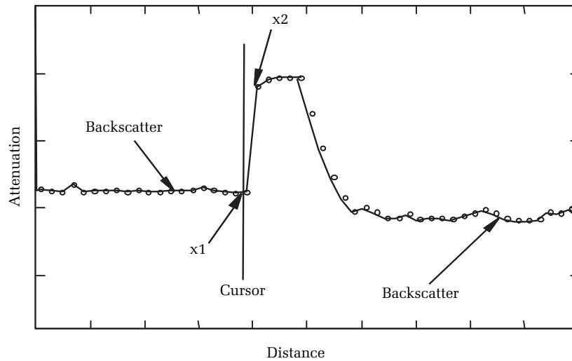
Figure 7.11. Locating the position of a reflective event in an OTDR's waveform. First, locate the position of sample point x1, which is the last sample point not on the event's rising edge. To this, add one-half of the sample spacing. This is the reflective event's position.
