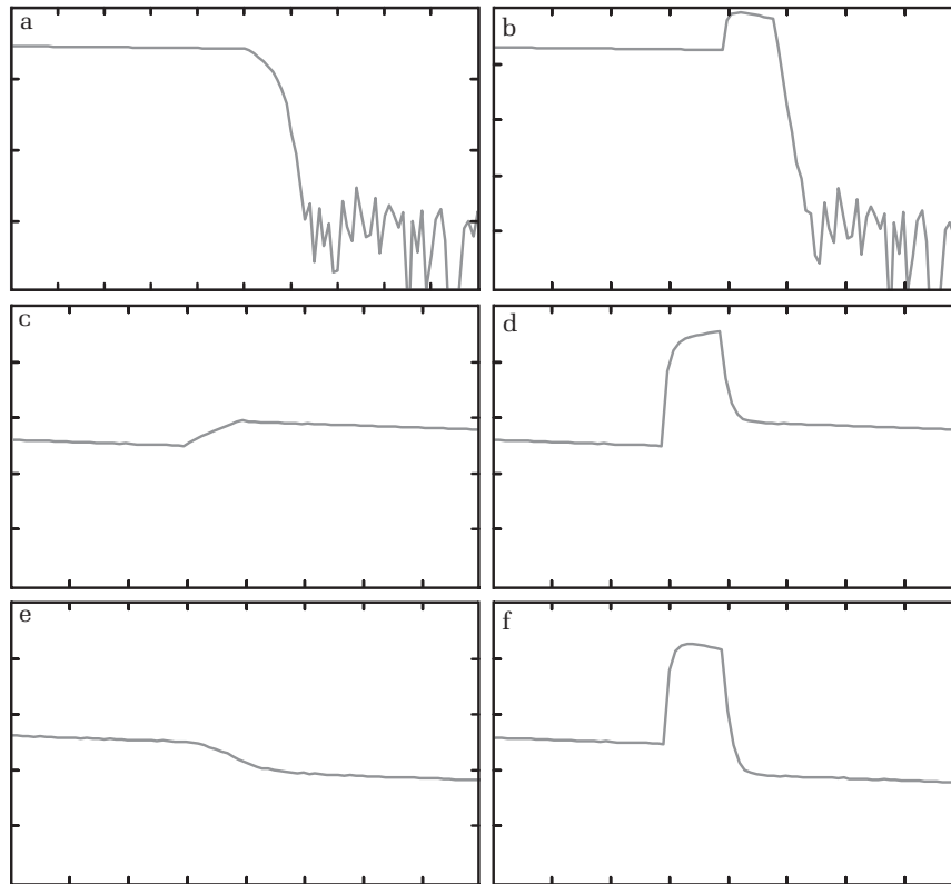
Figure 11.13. Types of isolated events: (a) Nonreflective fiber end, (b) reflective fiber end, (c) fusion splice with negative loss (gainer), (d) connector (reflective event) with negative loss (gainer), (e) fusion splice with positive loss, (f) connector (reflective event) with positive loss.
