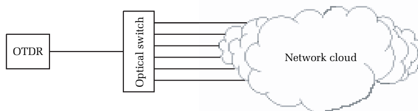
Figure 11.16. Remote OTDR system using an optical switch to periodically test various fibers in the optical network.
