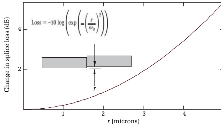
Figure 2.18. Coupling loss in single-mode fiber as a function of lateral misalignment. The mode-field diameter for both fibers is 4.5 \mu\text{m} .
