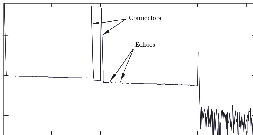
Figure 3.10. Two connectors spaced 200 meters apart. Light reflecting off these connectors results in a pair of echoes 200 meters after the last connector and spaced 200 meters apart. Observe that there is no loss associated with the echoes. The pair of connectors and the front panel each had -20 dB return loss. In this waveform, the pulse width is 20 meters, the fiber is single-mode, and the wavelength is 1310 nm.
