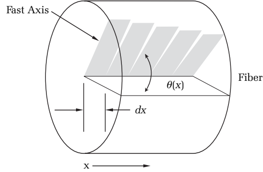
Figure 13.6. A length of fiber modeled as a series of arbitrary waveplates. Each differential waveplate is defined by its angle between the fast axis and the x-axis and its DGD. The state of output polarization is determined by the fiber's Jones matrix, which is the reverse product of the Jones matrices of the individual waveplates (see equation [13.5]).
