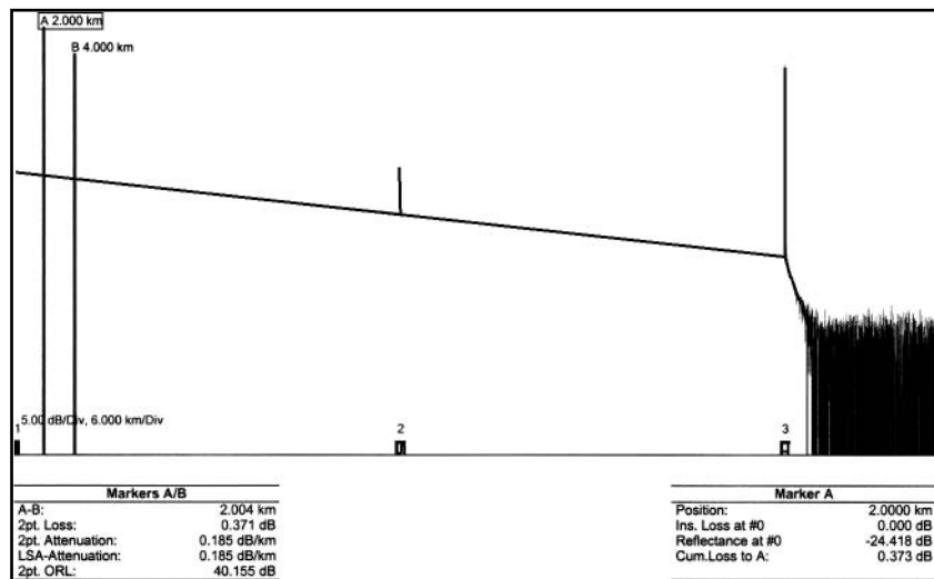
Figure 7.9. The OTDR trace of a mechanical splice is very similar to that of an APC (angled) fiber-optic connector. Both the APC and a mechanical splice with index-matching fluid or gel have ORL values of 50–60 dB.
