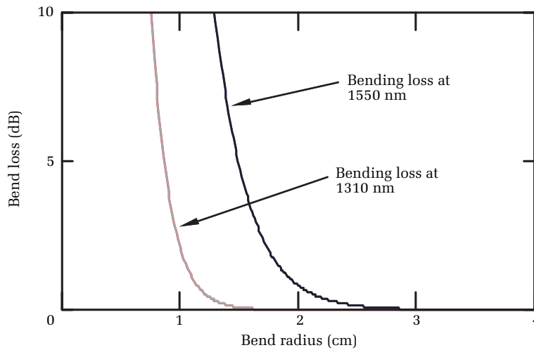
Figure 2.20. Bending loss as a function of bend radius (180° bend) using equation [2.30]. Loss at 1550 nm is considerably greater than it is at 1310 nm.
