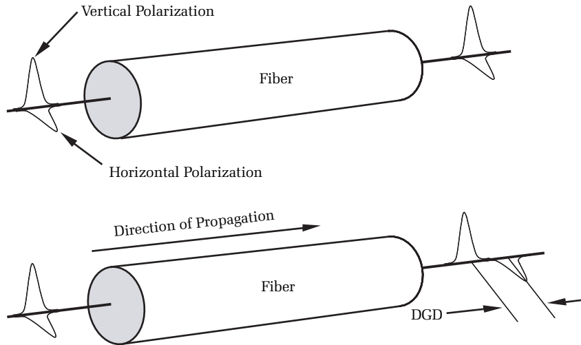
Figure 13.1. For a perfect fiber (top), the group velocities of the orthogonal polarization states are the same, so there is no pulse dispersion. Real fibers (bottom) always have some residual birefringence, resulting in slightly different group velocities for the orthogonal states. The difference in the arrival times of the pulses is the differential group delay, or DGD.
