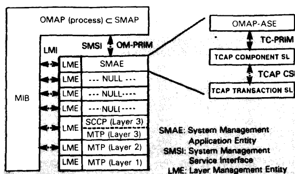
Fig. 15. SS7 management model.
