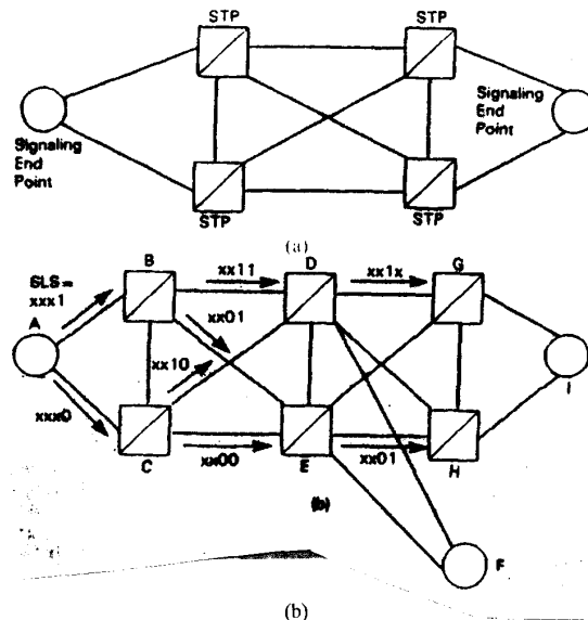
Fig. 7. Signaling network structure (ANSI).
