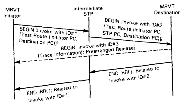
Fig. 16. MTP routing verification test with TCAP.
