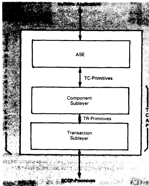
Fig. 11. Application layer structure.
