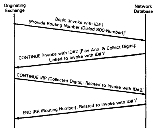
Fig. 14. 800 Service example using TCAP.
